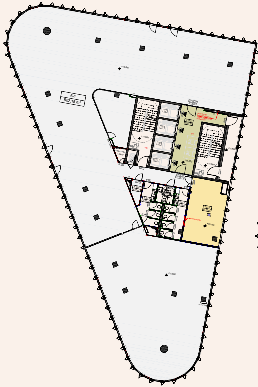
Tower: A
